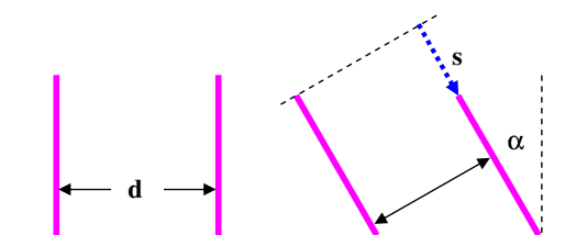
Figure 5. Schematic drawings of two parallel anthryl groups viewed along their long direction: left, without tilting; right, after introducing an off-plane tilting with an angle of \alpha , and thus resulting in a shift (or parallel-displacement) s essentially in the short direction of the anthryl groups along with a reduced perpendicular distance d \cos \alpha .
