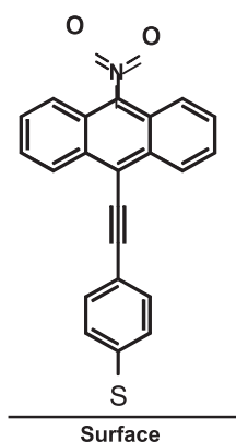
Chart 1. Side view of a MPNAA molecule adsorbed on the gold surface.
