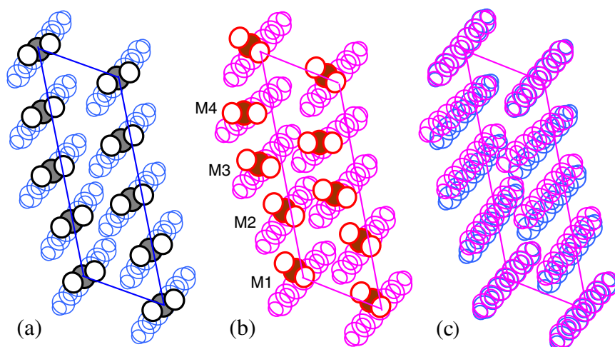
Figure 4. The models proposed (a) in [11] and (b) in the present study, as well as (c) the comparison of the two. For clarity, the nitro groups are not shown in (c).
